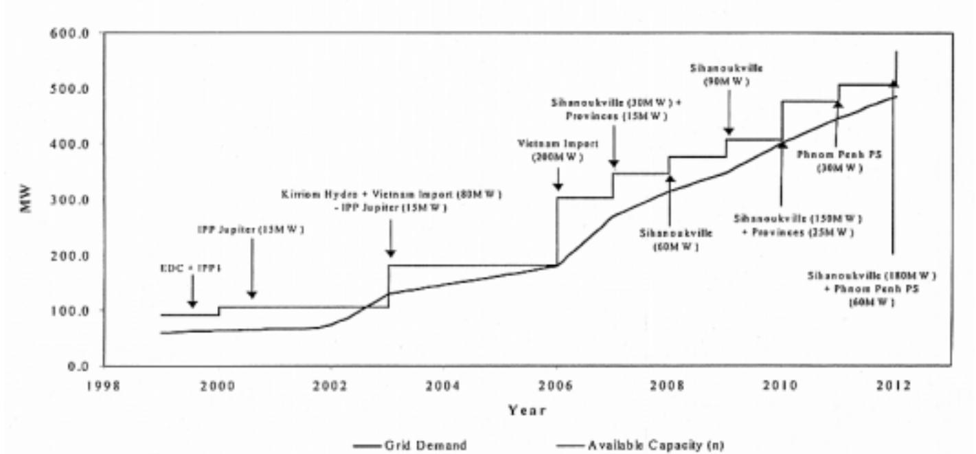
Figure I-1-1 Master Plan of Electric Power Generation and Transmission in Cambodia
